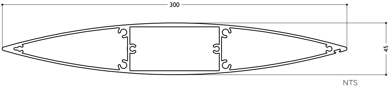
BLADE SPECIFICATIONS 300MM MAXI LOUVRE
